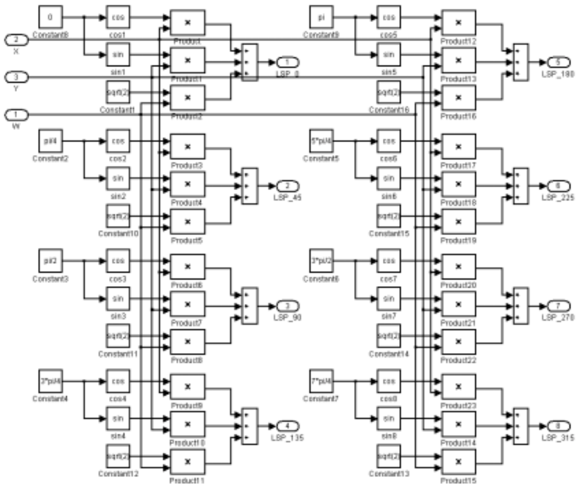
Fig. 5. Eight channel ambisonics decoder using Simulink building blocks.
