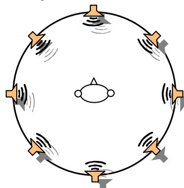
Fig. 4. Loudspeaker layout
