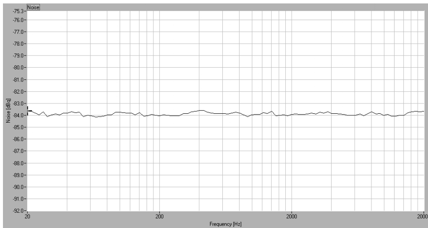
Fig. 10. Quasi peak rectified noise measurement of the system
