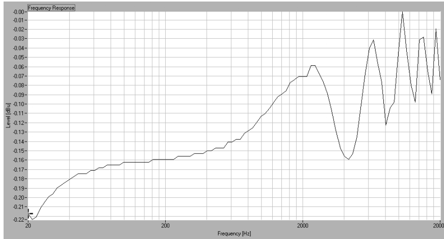
Fig. 9. Frequency response of the system
