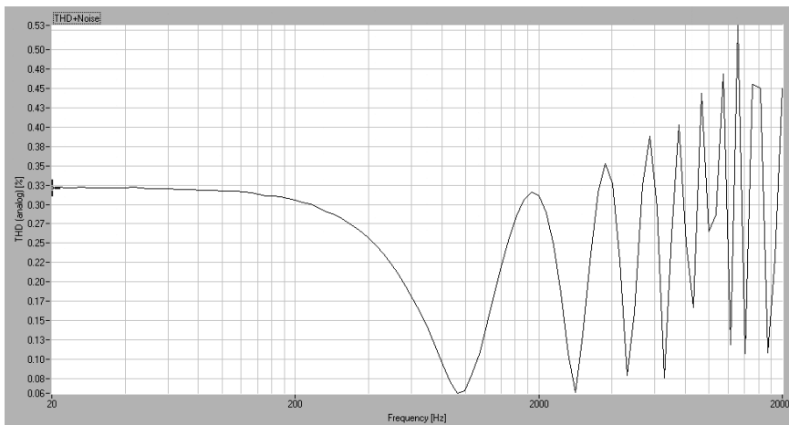
Fig. 11. THD + noise measurement of the system
