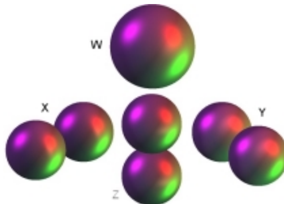
Fig. 3. Spherical harmonics forming B-format
